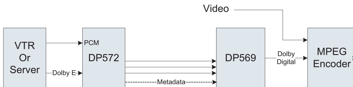
Figure 1-5 Play-out System
