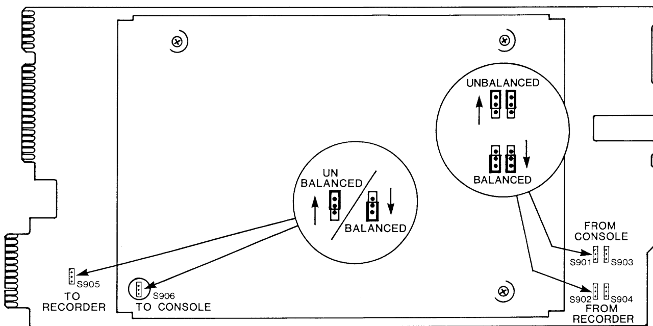
Figure 3-6 Cat. No. 431/531 Configuration Links
