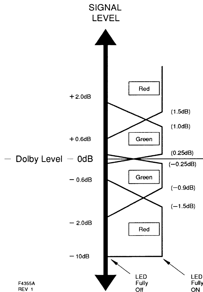
Figure 8-2b Range and Effects of Cross Fades Produced in LED Calibration Display of the Cat. No. 531
