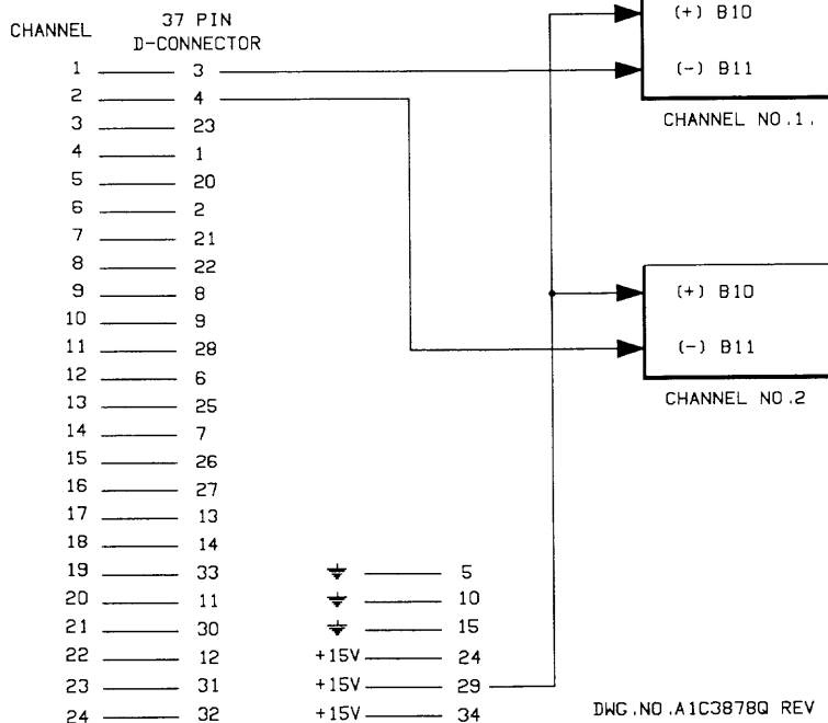
Figure 3-14 Remote Connection of XP/SRP Series Unit to Ampex ATR-116/124 Recorders
